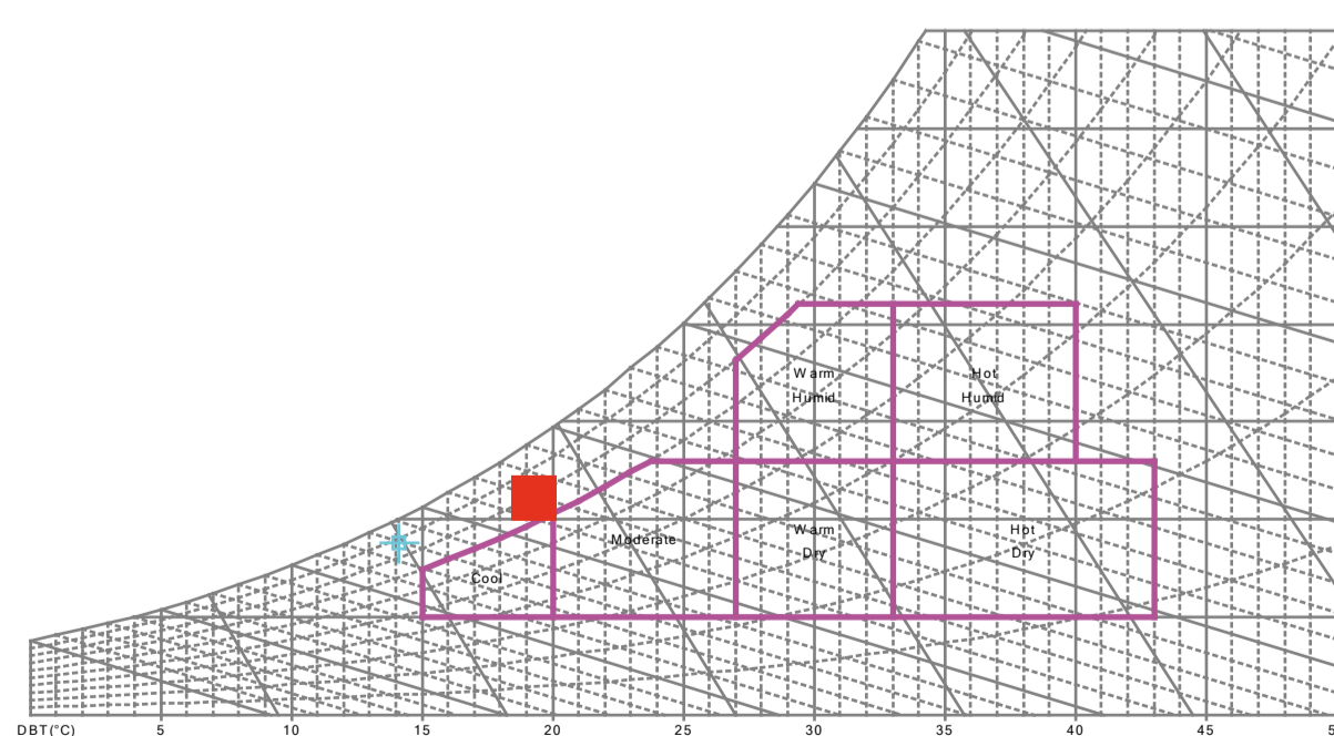
Psychrometric Chart Barometric Pressure: 101.36 kPa © Psychro Tech Ltd
